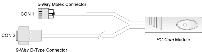
Figure 1. PC-Com Connectors
